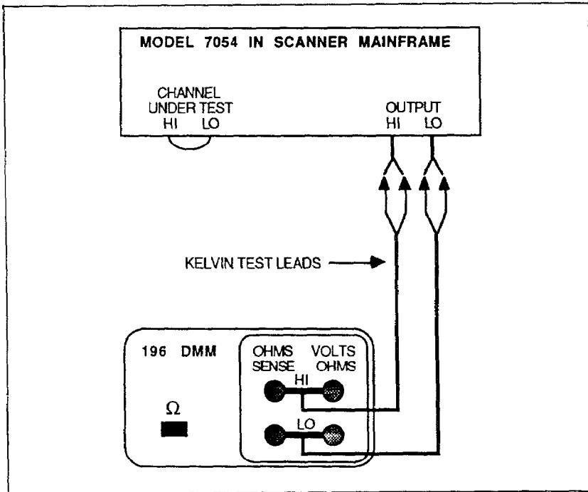
Figure 3-1. Contact Resistance
